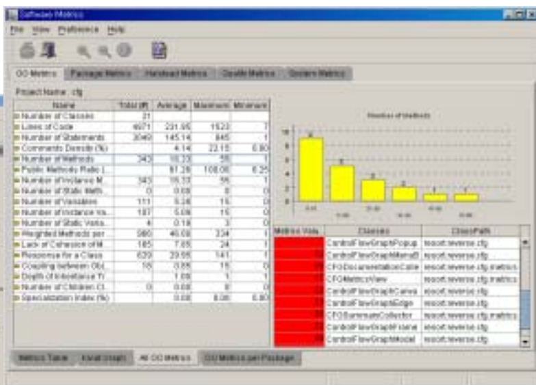
OO Metrics – Multi-level Statistical Metrics
