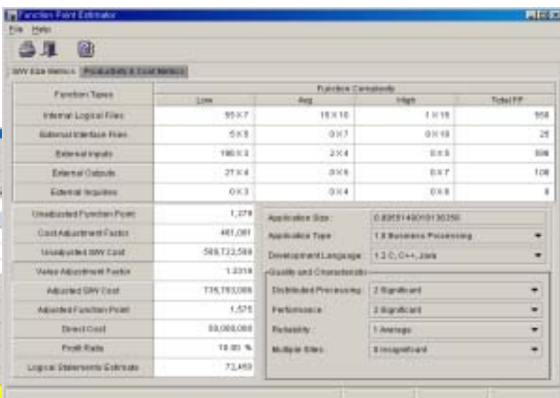
Function Point Estimator - SW Size Metrics
